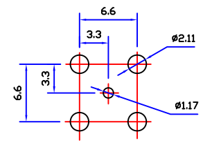
PCB HOLE CONFIGURATION RECOMMENDED PANEL CUTOUTS
